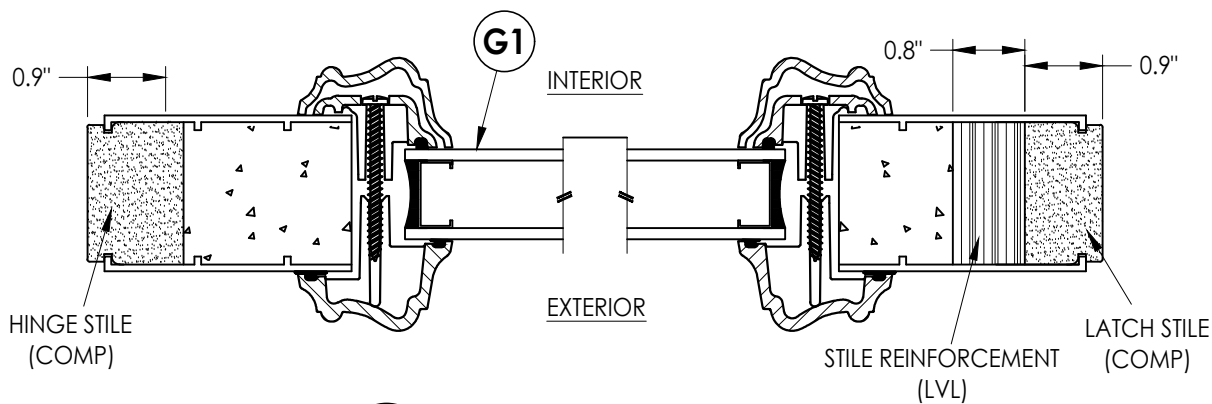
1 3 HORIZONTAL CROSS SECTION
