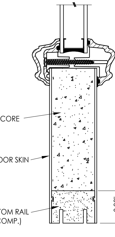
2 3 VERTICAL CROSS SECTION
