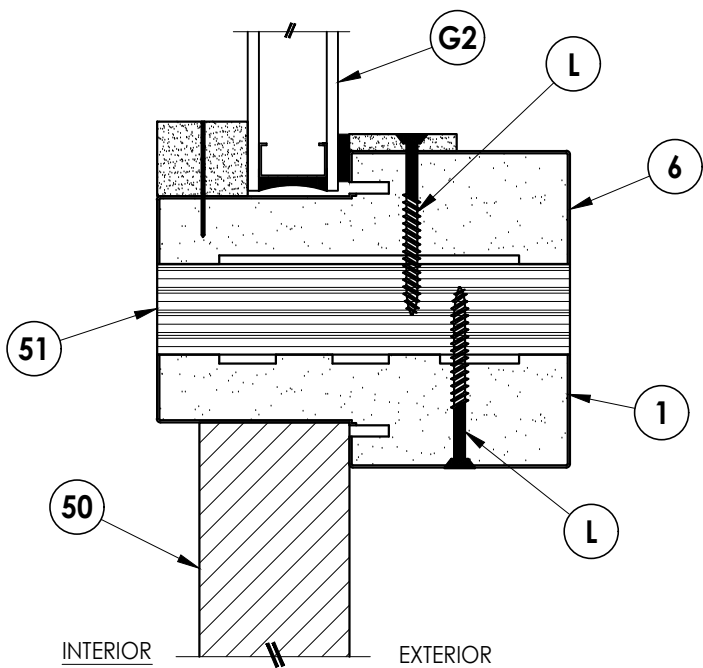
4 10 VERTICAL CROSS SECTION
