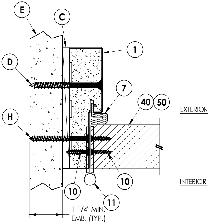
2 9 HORIZONTAL CROSS SECTION Inswing shown Direct to Masonry Construction
