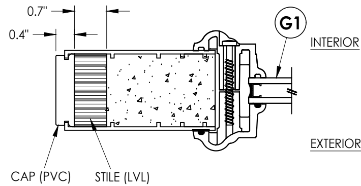
1 HORIZONTAL CROSS SECTION
