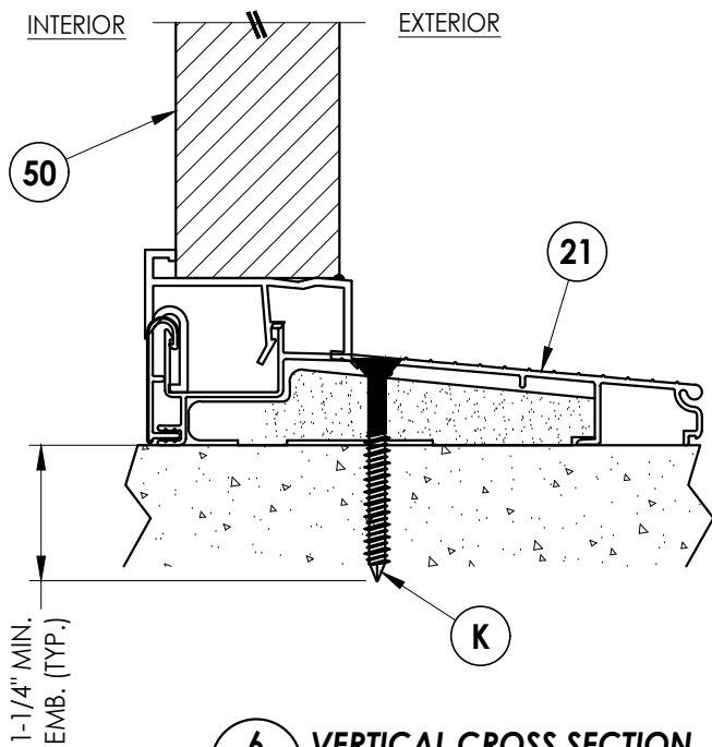
6 10 VERTICAL CROSS SECTION Inswing sill
