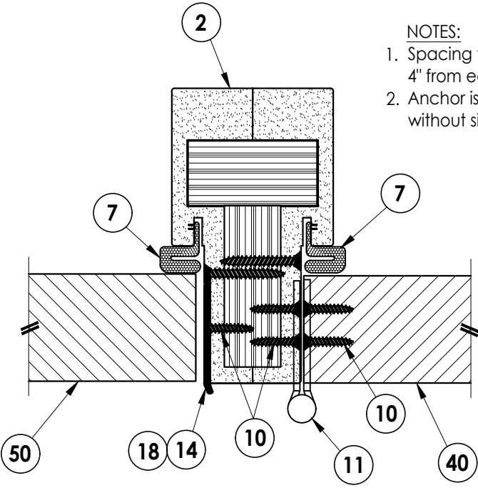
2 10 HORIZONTAL CROSS SECTION
