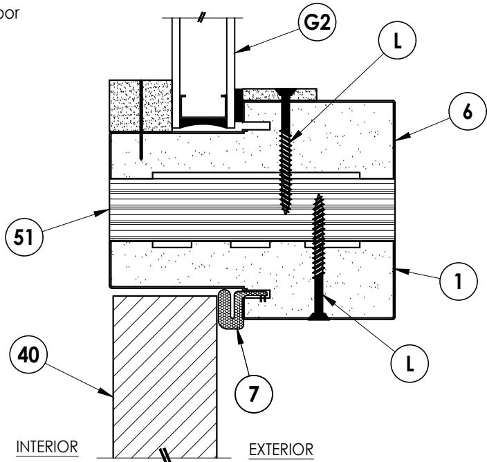
3 10 VERTICAL CROSS SECTION
