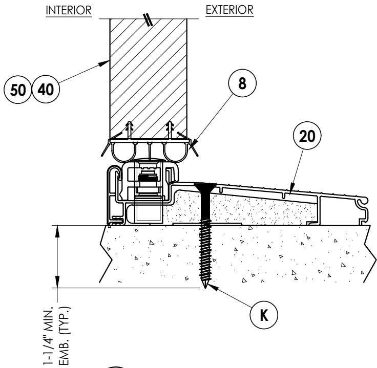
5 10 VERTICAL CROSS SECTION Inswing sill
