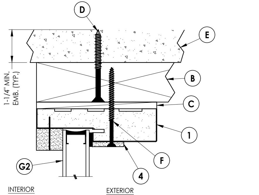
1 VERTICAL CROSS SECTION Inswing shown 2X Buck Construction
