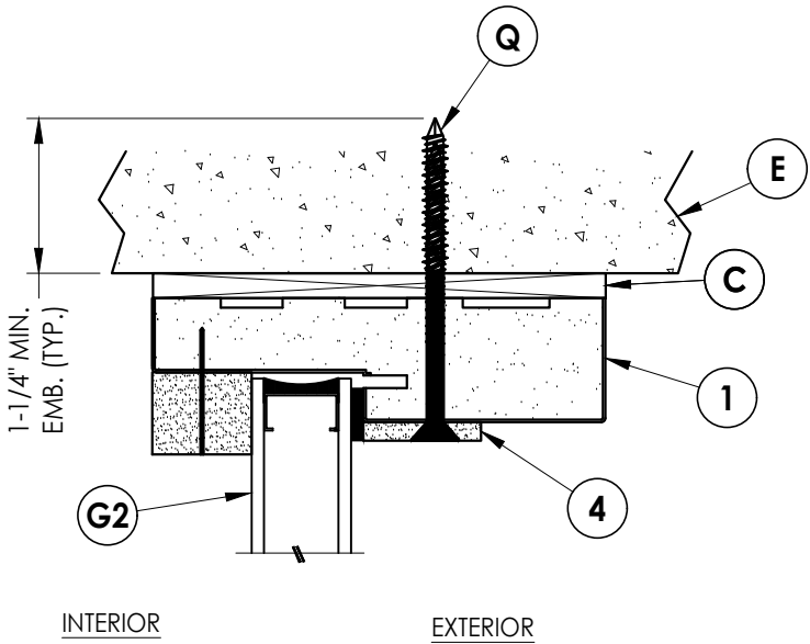
1 9 VERTICAL CROSS SECTION Inswing shown Direct to Masonry Construction
