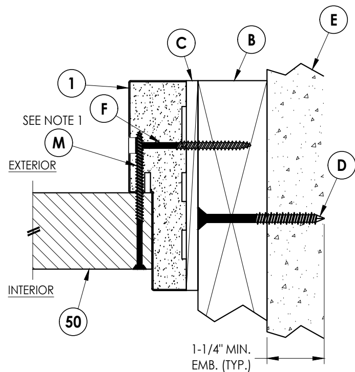
4 HORIZONTAL CROSS SECTION Inswing shown 2X Buck Construction
