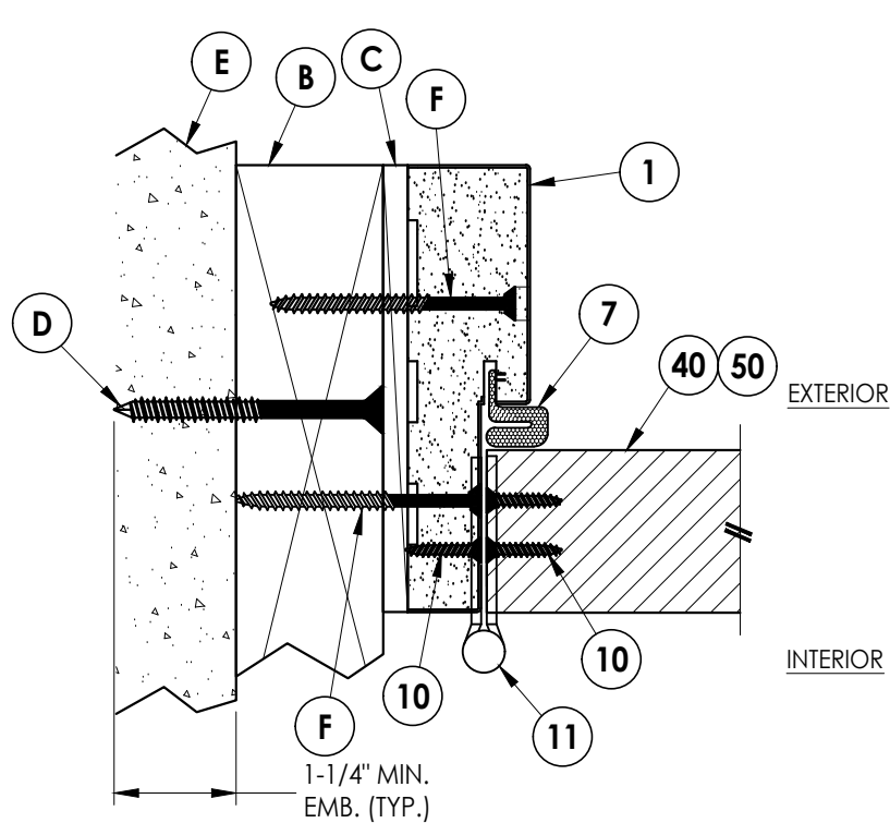
2 HORIZONTAL CROSS SECTION Inswing shown 2X Buck Construction
