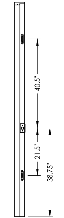
STRIKE MULLION Multi-point Lock (Vented Sidelite)
