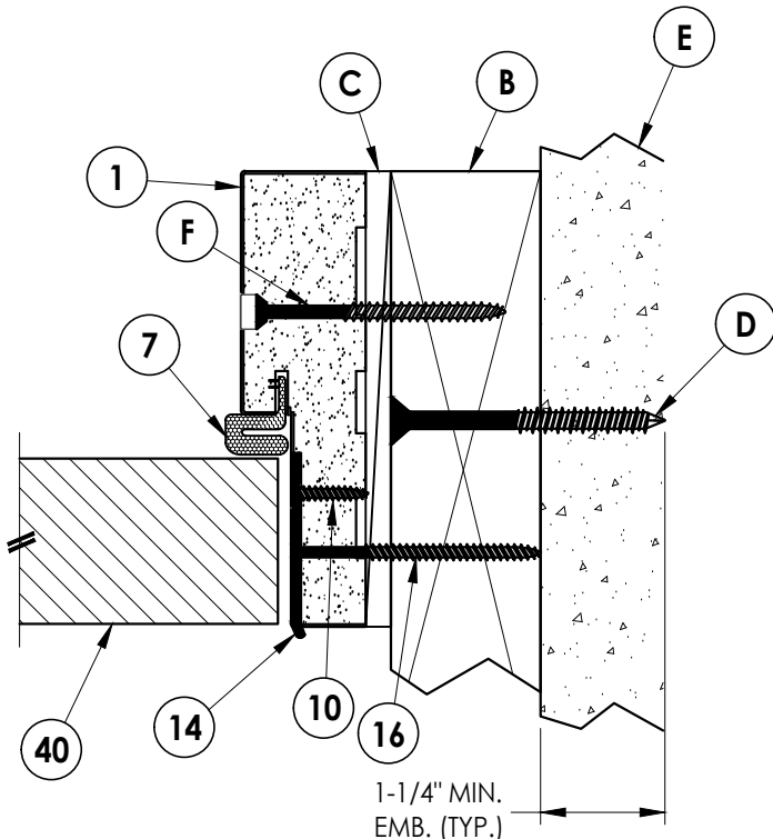
3 HORIZONTAL CROSS SECTION Inswing shown 2X Buck Construction
