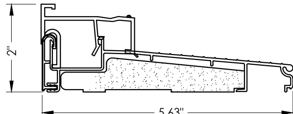
21 INSWING THRESHOLD w/ SIDELITE ADAPTER Endura (Z-Series)
