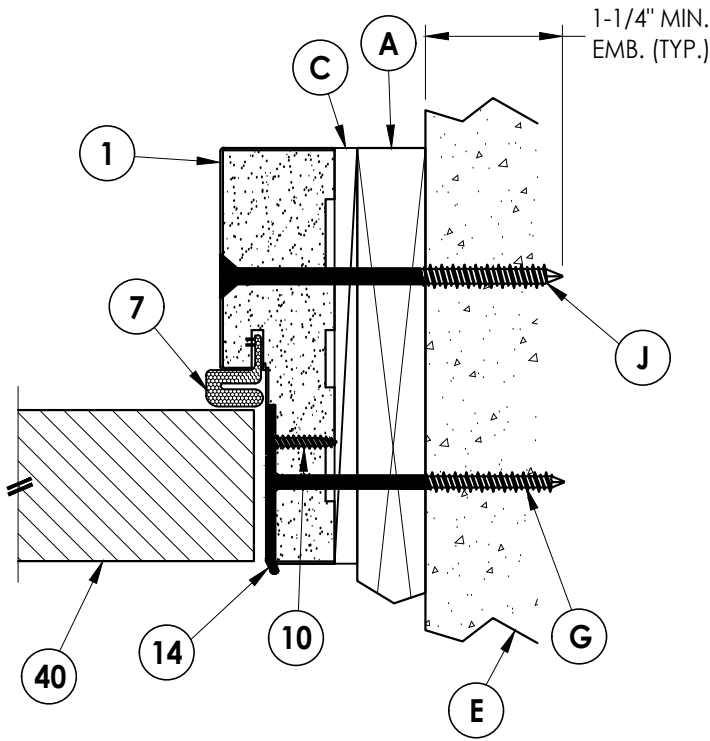
3 8 HORIZONTAL CROSS SECTION Inswing shown 1X Buck Construction
