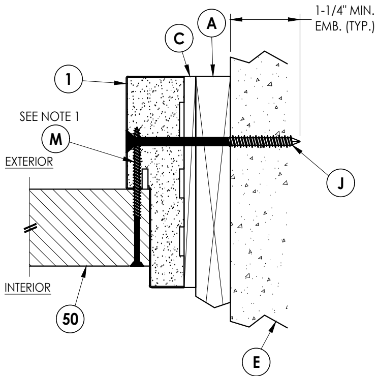
4 8 HORIZONTAL CROSS SECTION Inswing shown 1X Buck Construction
