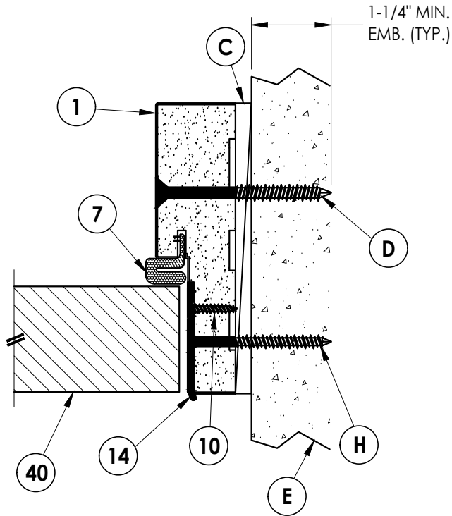
3 9 HORIZONTAL CROSS SECTION Inswing shown Direct to Masonry Construction
