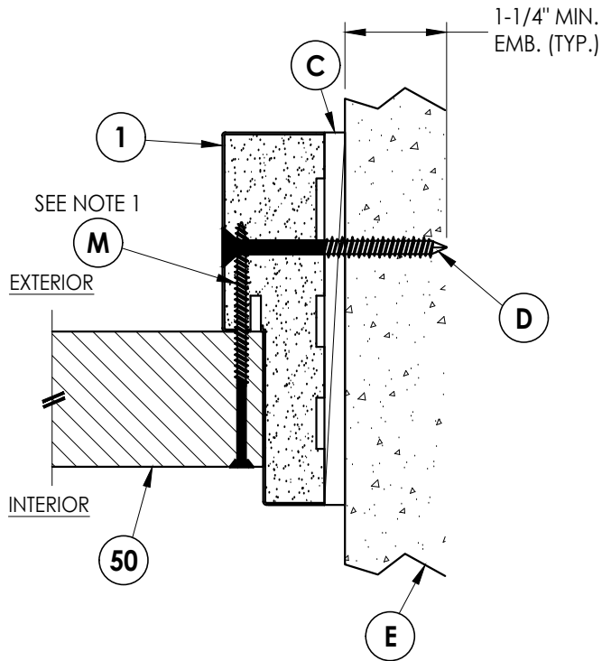
4 9 HORIZONTAL CROSS SECTION Inswing shown Direct to Masonry Construction
